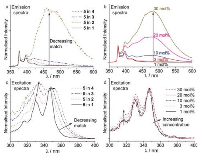
Fig. 3 Fluorescence emission (a–b, \lambda_{\text{exc}} = 330 nm) and excitation (c–d, \lambda_{\text{em}} = 487 nm) spectra of 3 mol% of 5 mixed with different polymers (a and c) or different mol% of 5 in the matching polymer 1 (b and d). The emission (excitation) spectra were normalized to the peak at 377 (347) nm.
