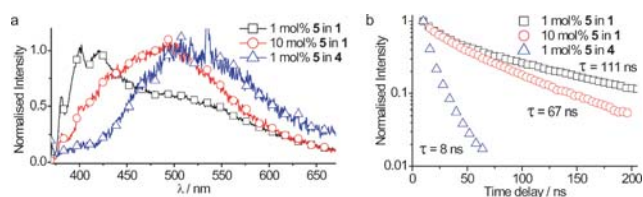
Fig. 4 Fluorescence spectra ( \lambda_{\text{exc}} = 358 nm) of thin films containing 1 and 10 mol% of 5 in 1 and 1 mol% of 5 in 4 at 10–30 ns delay time after the excitation pulse (a) and decay of the emission between 400 and 700 nm of these films after the first 10 ns (b).
