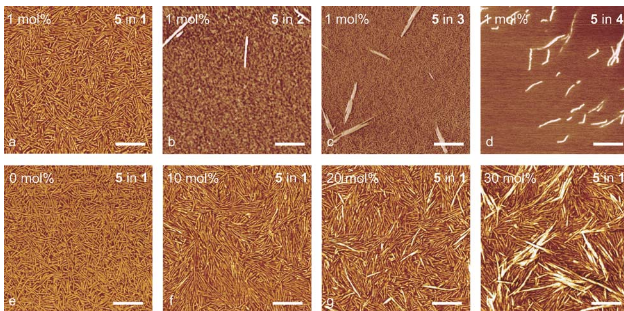
Fig. 2 Intermittent contact mode AFM phase images. Top: thin films of 1 mol% 5 in 1 (a), 2 (b), 3 (c) and 4 (d). Bottom: thin films of 0 (e), 10 (f), 20 (g) and 30 (h) mol% 5 in 1 . Samples in a and e–h were annealed for 30 min at 110 °C prior to AFM imaging. The scale bar is 200 nm in all images.
