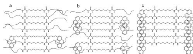
Fig. 1 Bisurea stacking. (a) 5 at low concentration in 1 . (b) 5 at high concentration in 1 . (c) Self-assembled, phase-separated stack of 5 .
