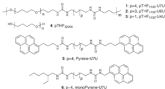
Scheme 1 Set of molecules used for the mixing experiments.
